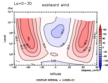
Figure 64: U at L_S=0^\circ-30^\circ by DC-PAM
